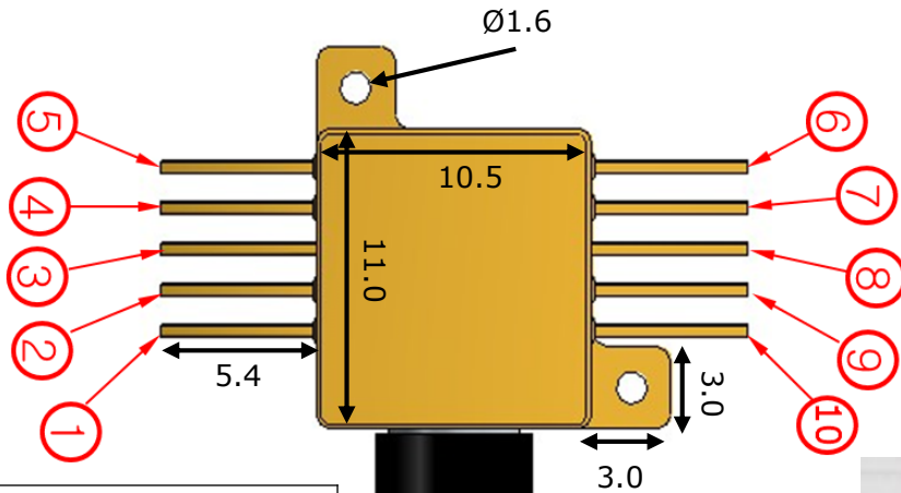
Pin Configuration
